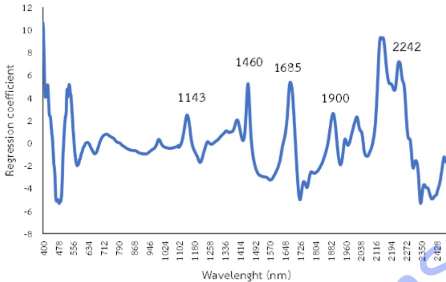
Figure 3 Regression coefficient for calibration model to predict curcuminoid contents in Turmeric powder samples
