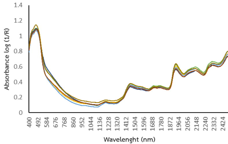
Figure 1 The original NIR spectra of Turmeric powder samples at wavelength 400–2500 nm.
